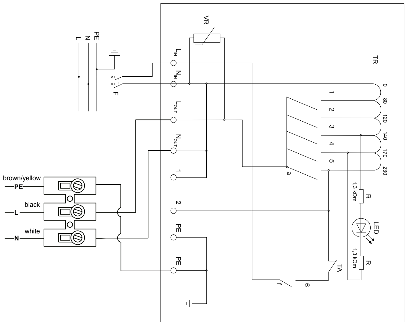
Connection diagram with HRB speed controller
